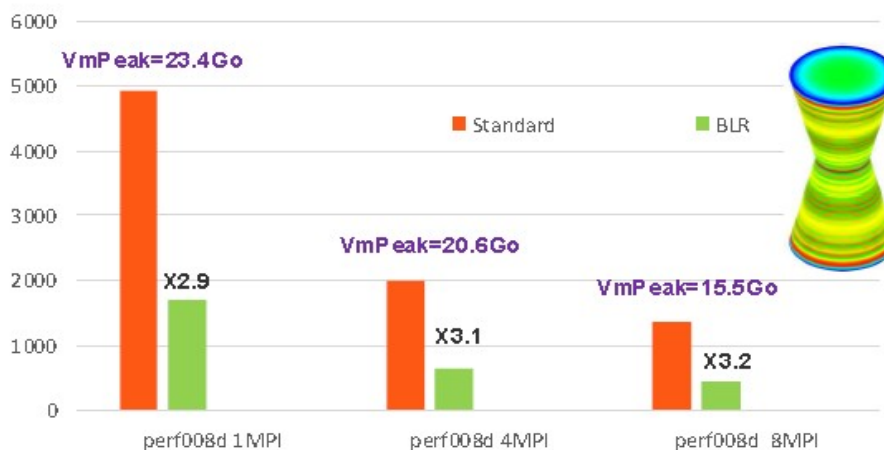
Figure 7.2-2: Example of profits gotten by compressions low-rank on the case benchmark perf008d (parameters by default, management memory in OOC, N=2M , NNZ=80M , Facto\_METIS4=7495M , conditionnement=10^7 ). One traces, according to the number of activated processes MPI, the times elapsed spent by all the stage of resolution of system linear in Code_Aster v13.1, his peak RAM report, as well as the factor of acceleration gotten by BLR.
