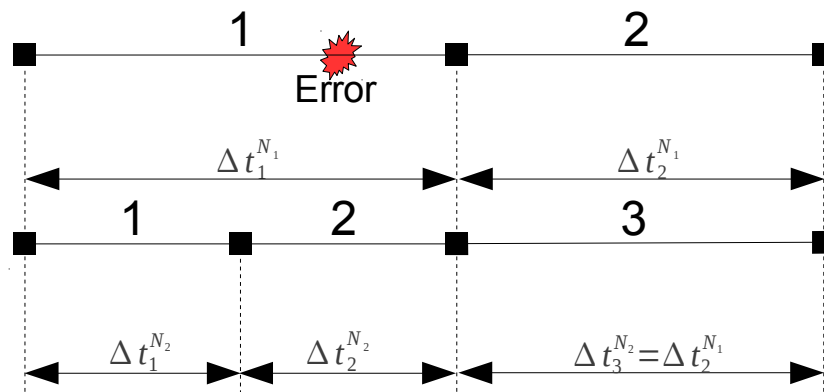
Figure 3-2: Cutting in mode HANDBOOK with SUBD_PAS=2
