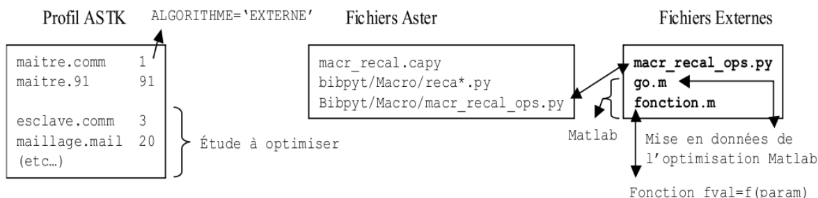
Figure 7.2.1-a: MACR_RECAL "External algorithm"
