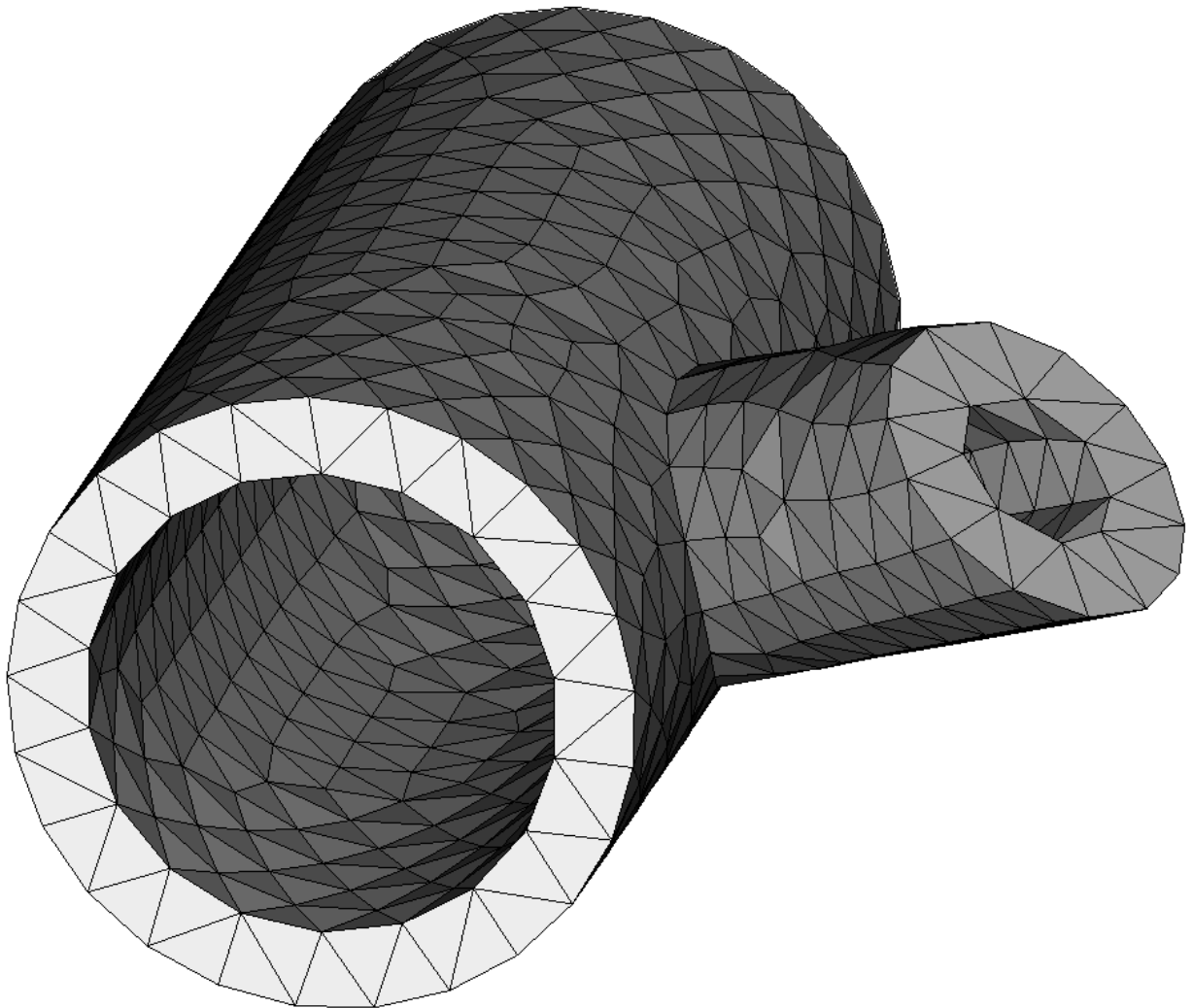
Figure 3.2.1-1.: Maillage initial
