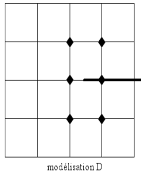
Figure 5-a : Enrichment in a zone close to the bottom of crack
