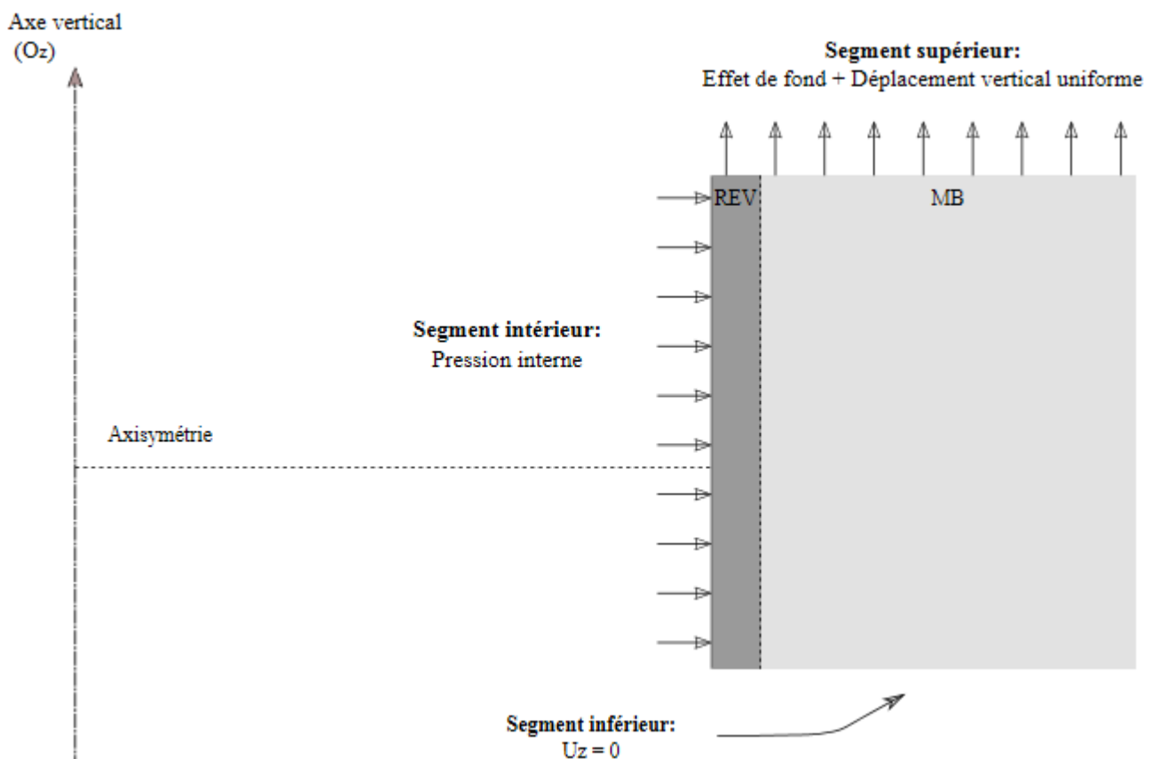
Figure 1.3-b: Mechanical problem considered
