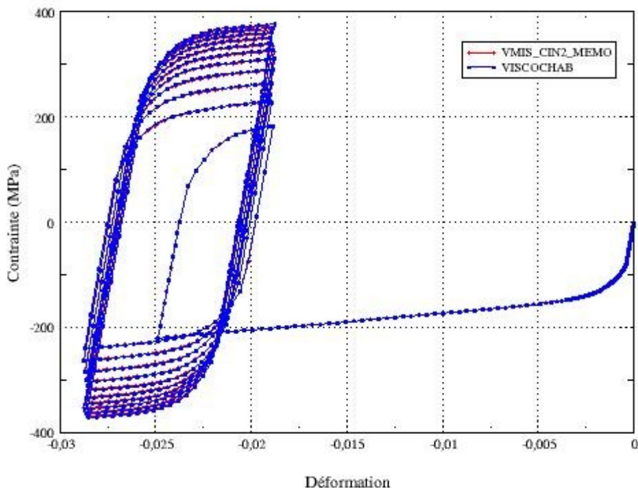
Essai cyclique DEPS= \pm 0.5\%
