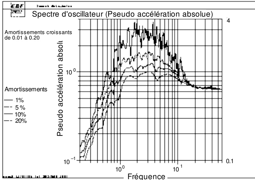
Figure 1.2.3-a: Spectrum of oscillator in pseudonym absolute acceleration
