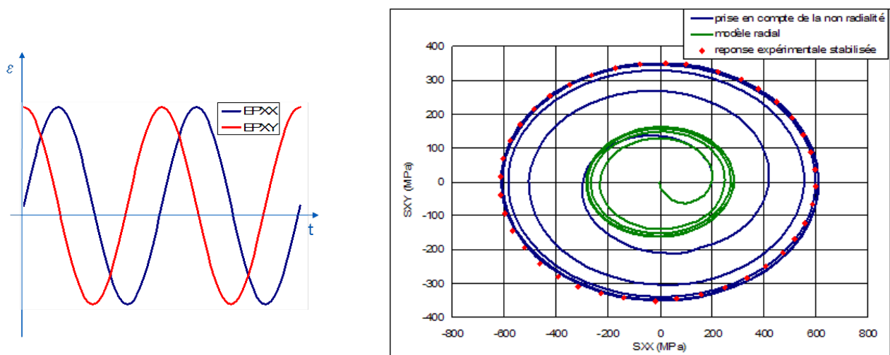
Figure 1.7-1 : Effect of on-work hardening under nonradial multiaxial loading
