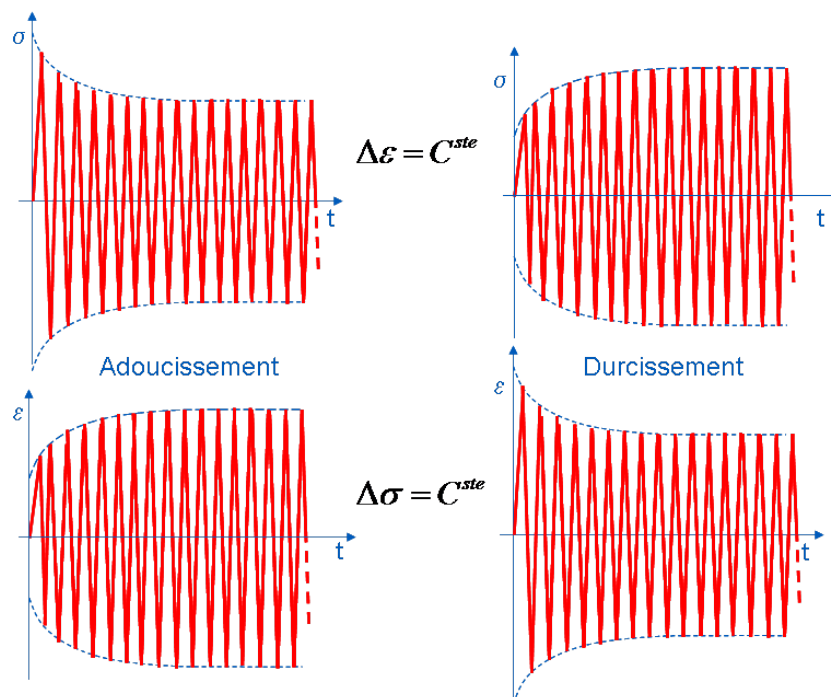
Figure 1.4-2 : Hardening and cyclic softening
