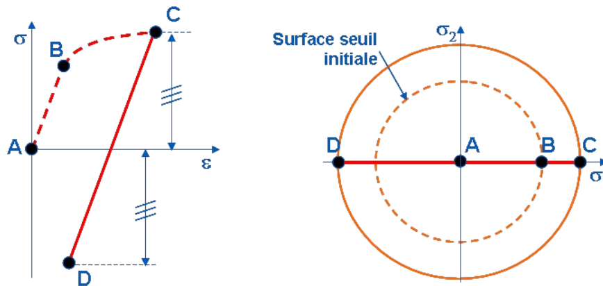
Figure 1.8-1 : Isotropic work hardening
