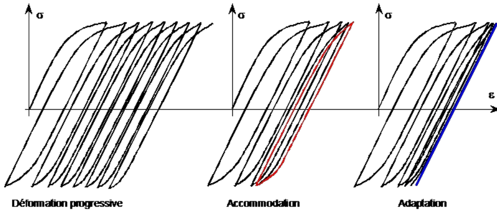
Figure 1.4-1 : Stabilization of the cyclic answer of material
