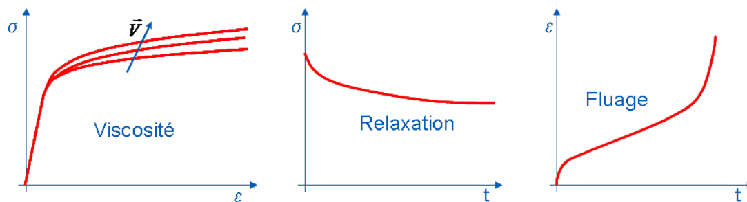
Figure 1.3-1 : Manifestation of viscosity according to the nature of the request
