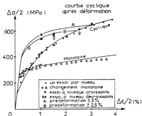
Figure 1.6-1 : The ratchet effect of work hardening
