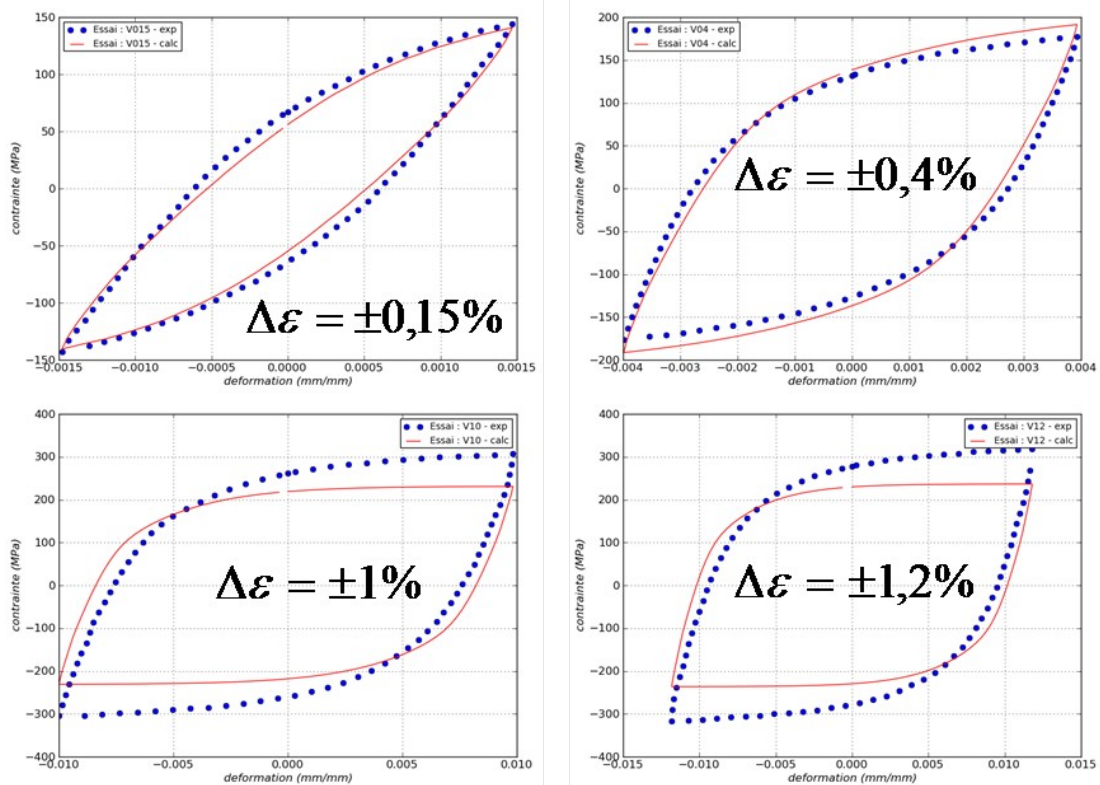
Figure 2-4 : Estimate of the robustness of a law of behavior in the event of extrapolation out of its field of validity.
