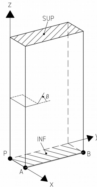
Figure 1.3-a: boundary conditions and loadings
